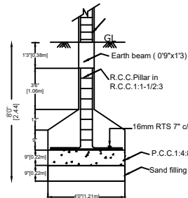
FOUNDATION DETAILS
