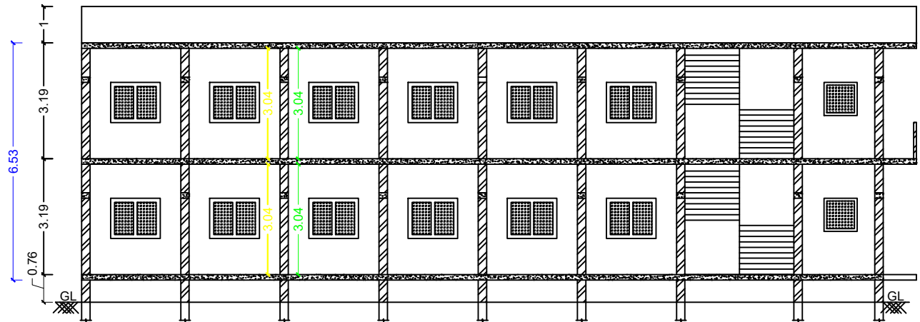
SECTION AT A1-A1
