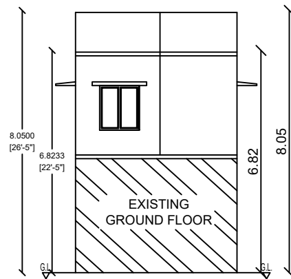
ELEVATION ON WEST
