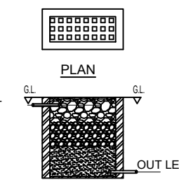
RAINWATER STORAGE PIT DETAILS
