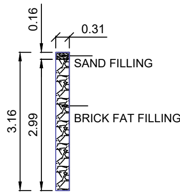
DETAILS OF PERCULATION PIT
