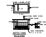
SEPTIC TANK
