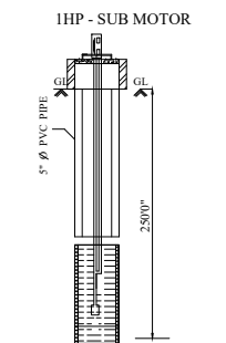
BOREWELL DETAILS
