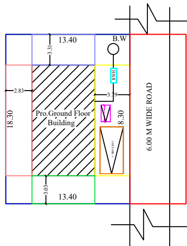
SITE PLAN
