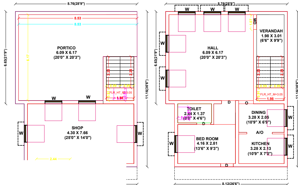
FLOOR-FIRST
