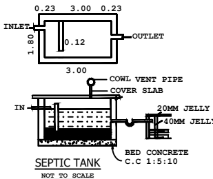
SEPTIC TANK
