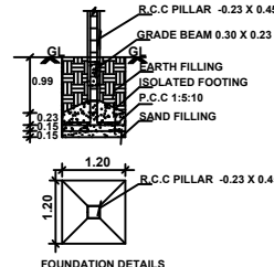
FOUNDATION DETAILS
