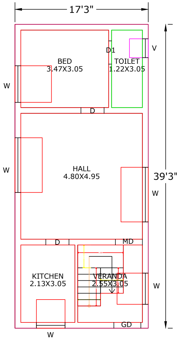
PRO.GROUND FLOOR PLAN
