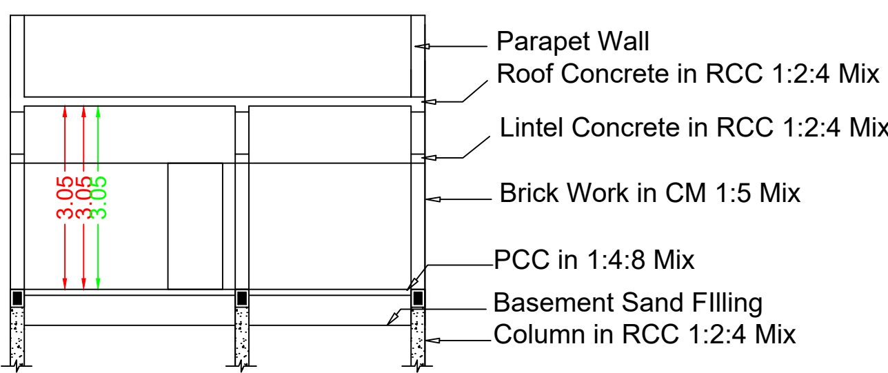
Section RR
