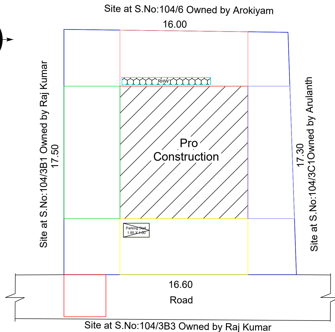
Site Plan
