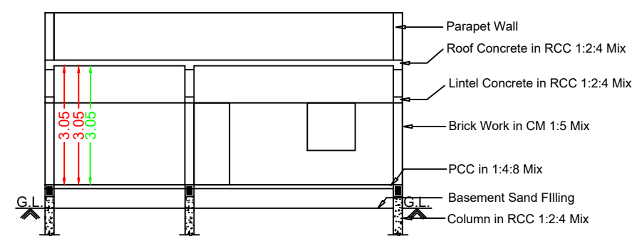
Section RR
