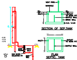
RAIN WATER HARVESTING SYSTEM RWHP CAPACITY :1000LTRS
