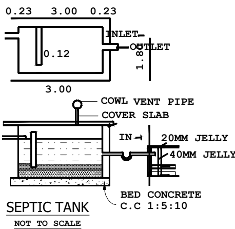
SEPTIC TANK
