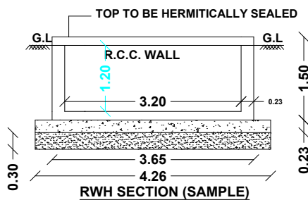
RWH SECTION (SAMPLE)
