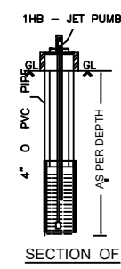
Section RR
