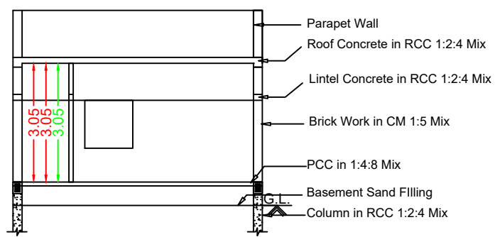
Section RR
