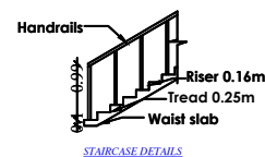
STAIRCASE DETAILS
