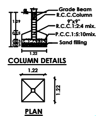
PLAN
