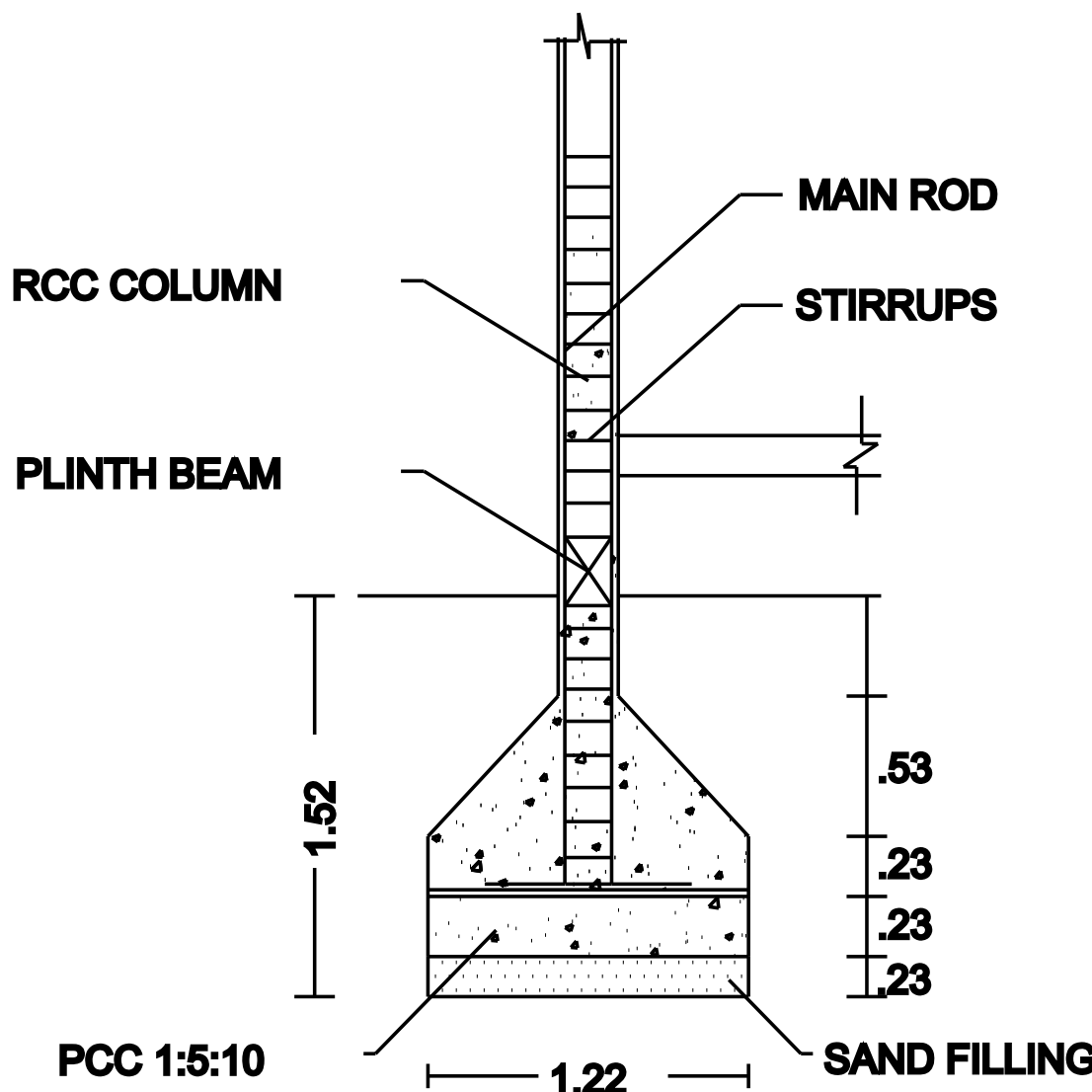
COLUMN DETAILS
