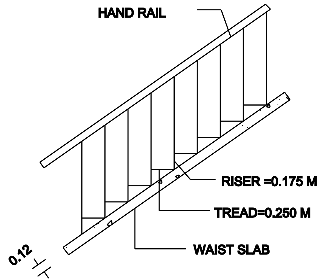
STAIRCASE DETAILS
