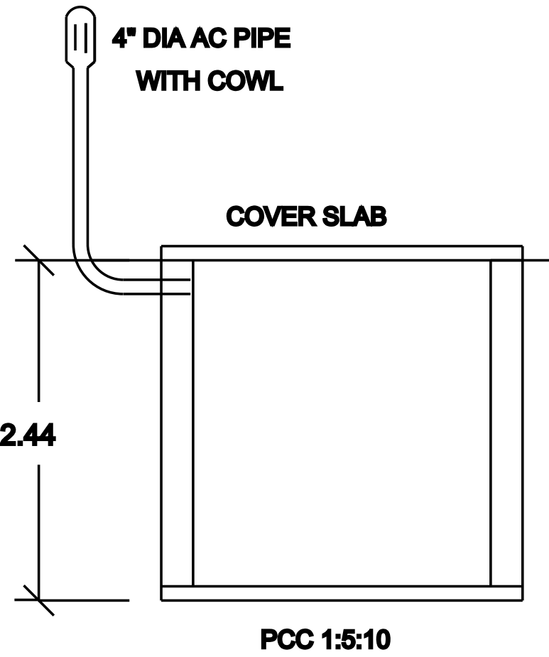
SEPTIC TANK
