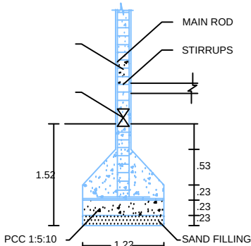
COLUMN DETAILS
