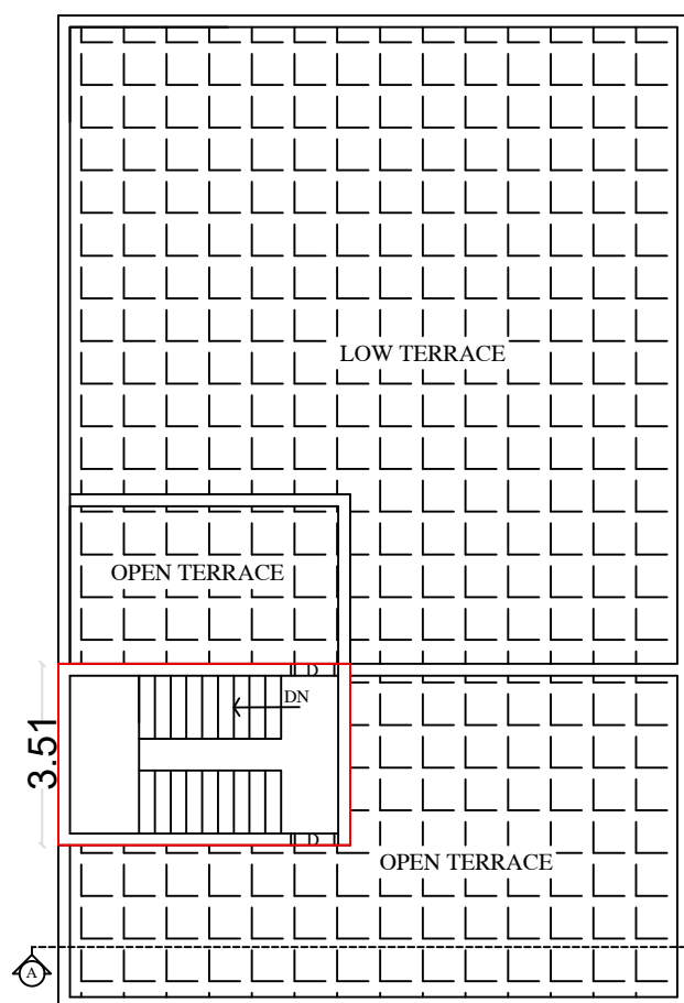
HEAD ROOM FLOOR PLAN
