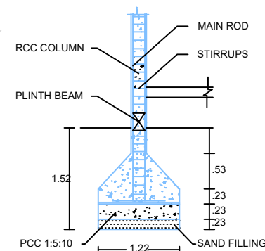
COLUMN DETAILS
