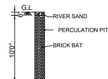
PERCULATION PIT
