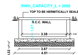
RWH SECTION (SAMPLE)
