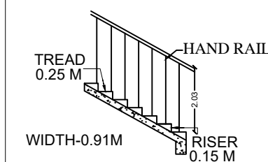
STAIRCASE DETAILS
