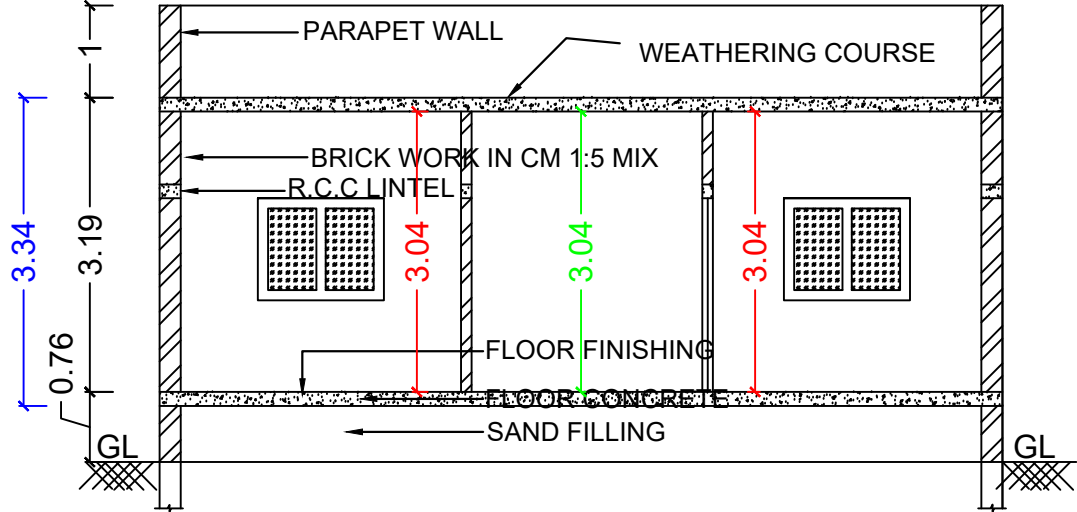
SECTION AT A1-A1
