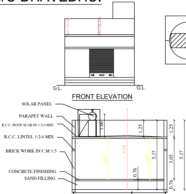
SECTION
