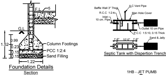
SECTION
