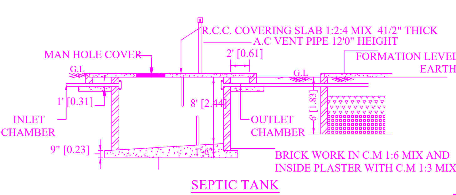
SEPTIC TANK
