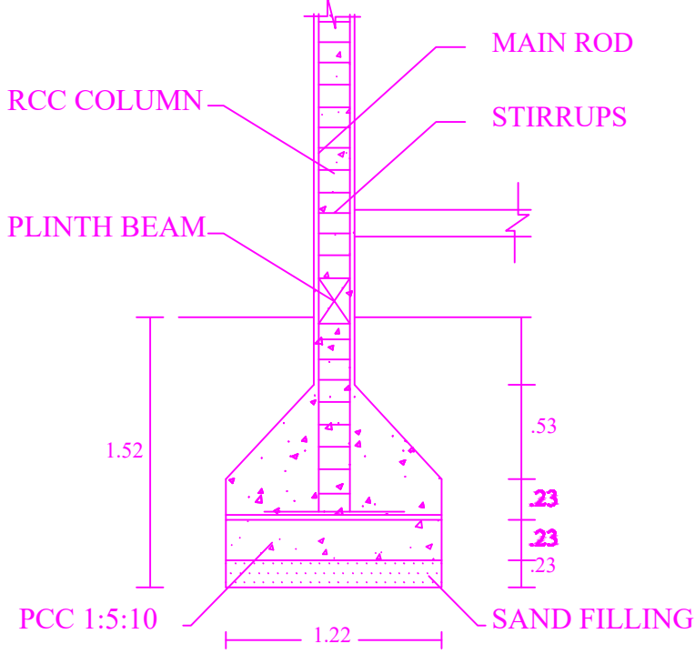
COLUMN DETAILS
