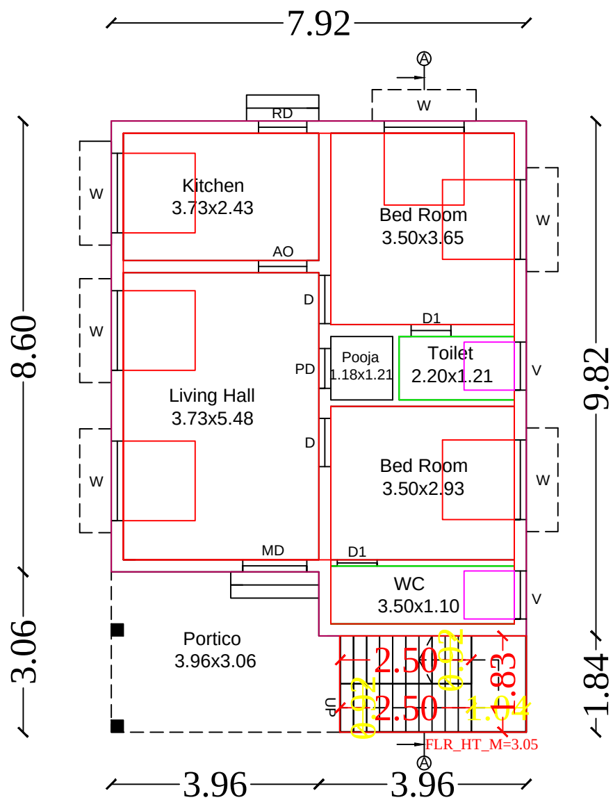
Ground Floor
