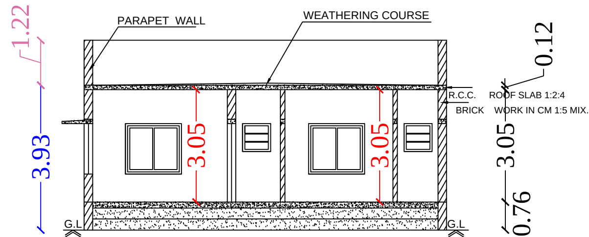
Section on-"AA"
