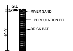
PERCULATION PIT
