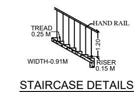
STAIRCASE DETAILS
