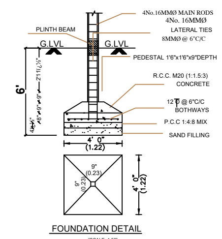
FOUNDATION DETAIL
