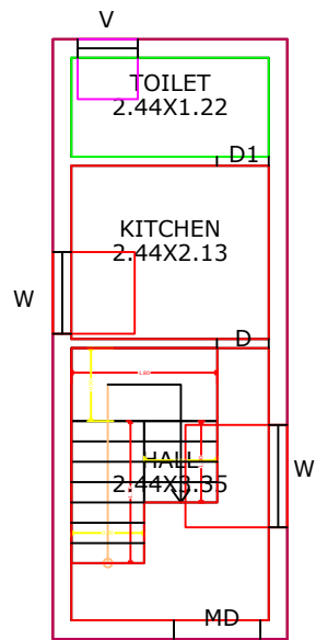
PRO.GROUND FLOOR PLAN
