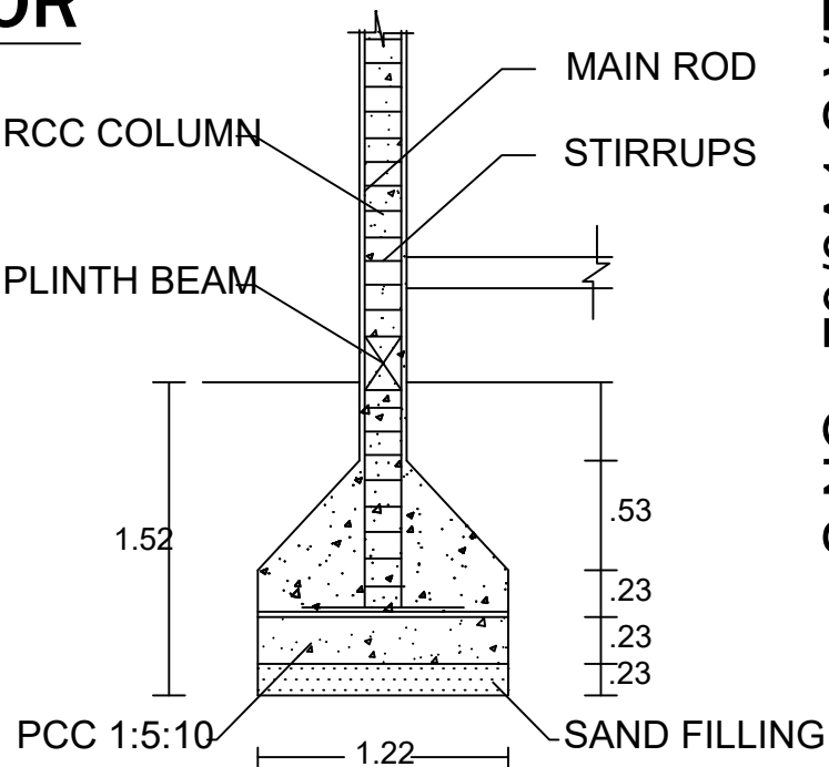
COLUMN DETAILS
