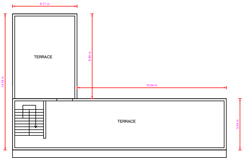
TERRACE PLAN
