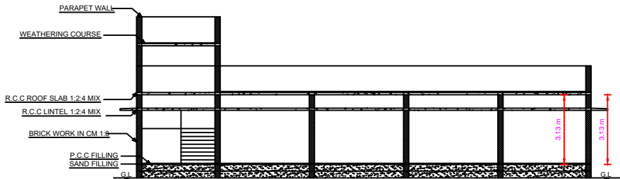
SECTION
