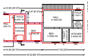
GROUND & EXG-GROUND FLOOR PLAN
