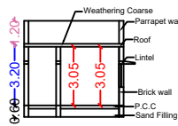
SECTION ON 'RP'
