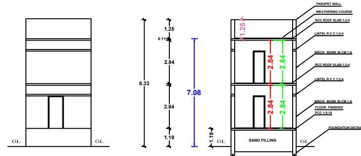
FRONT ELEVATION
