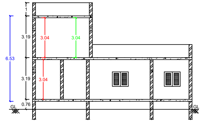
SECTION AT A1-A1
