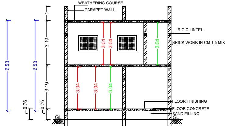
SECTION AT A1-A1
