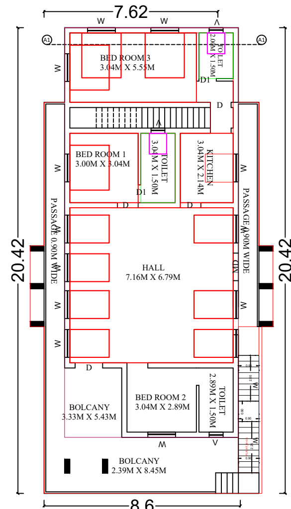
FIRST FLOOR PLAN BLOCK -2
