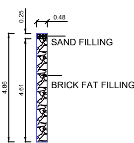
DETAILS OF PERCOLATION PIT
