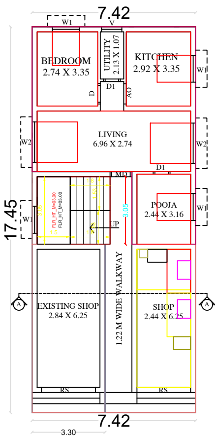
ADDITIONAL GROUND FLOOR PLAN
