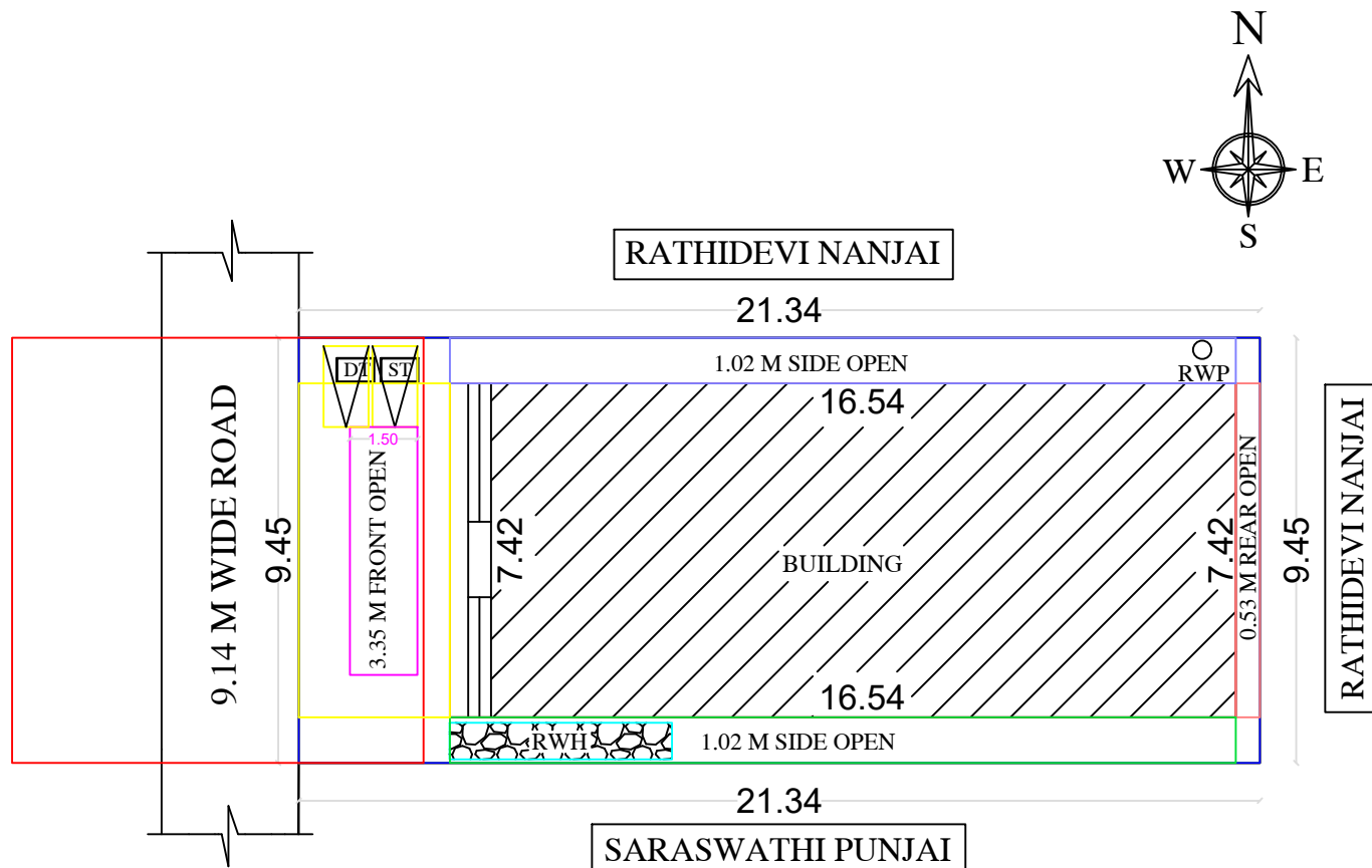
SITE PLAN
