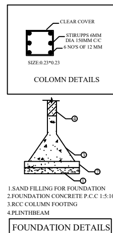
FOUNDATION DETAILS
