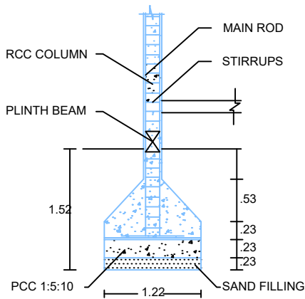
COLUMN DETAILS
