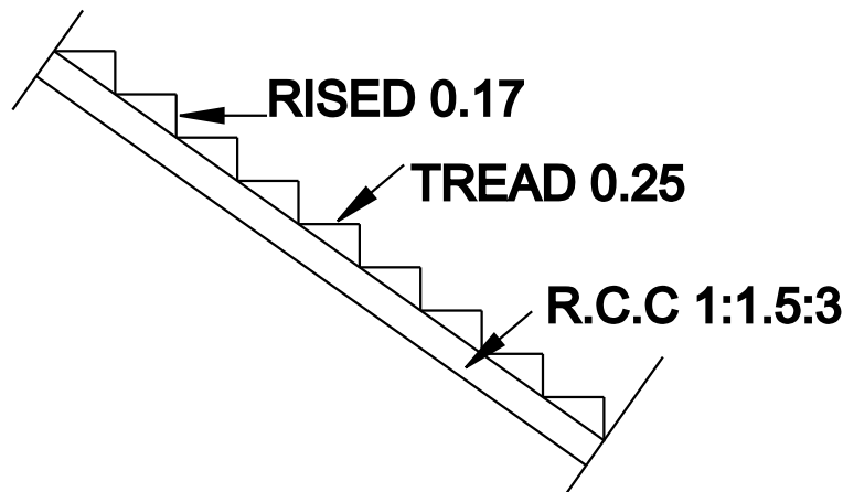
STAIRCASE DETAILS
