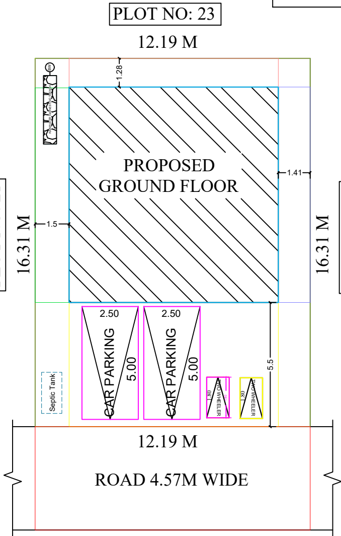
SITE PLAN (1:100)
