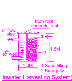
inwater Harvesting System
