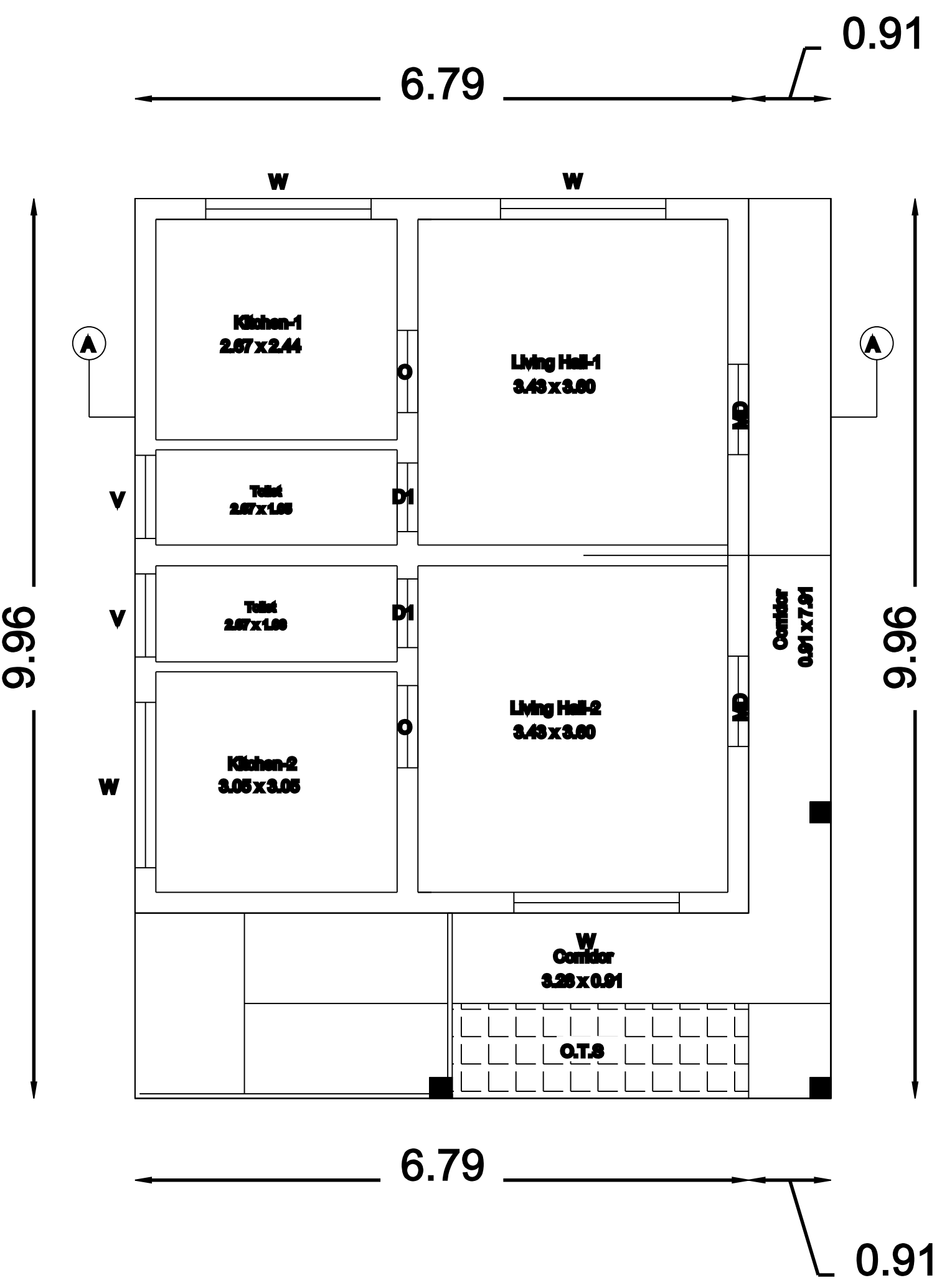
First Floor
