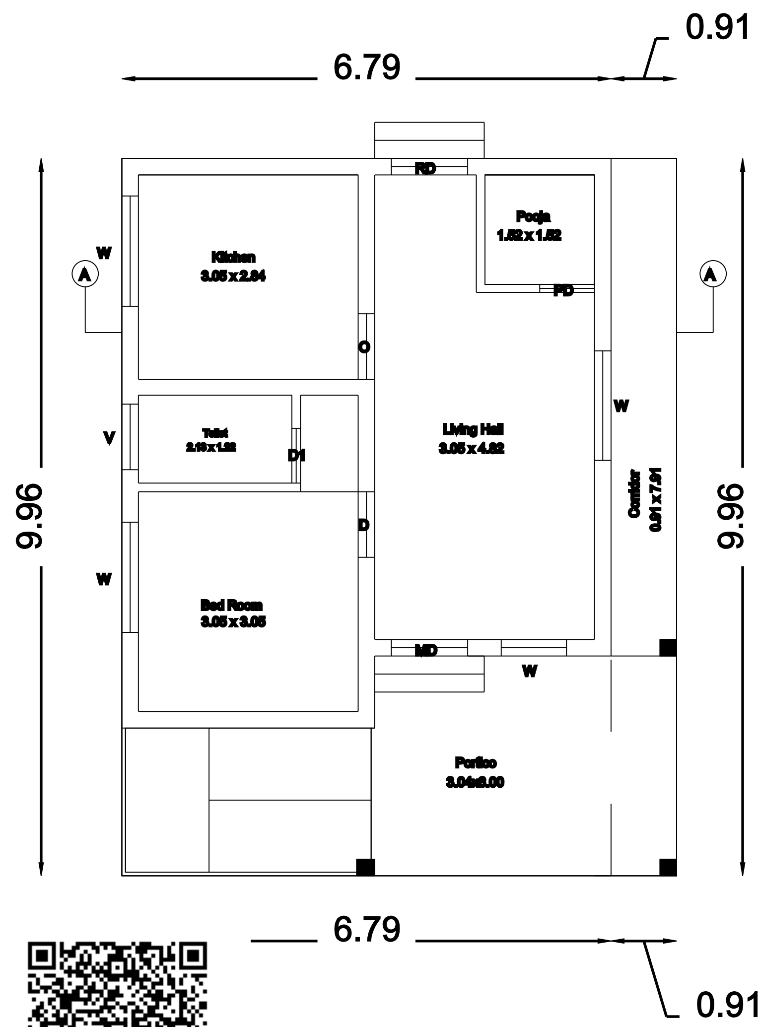
Ground Floor
