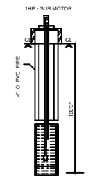
Bore Well Details
