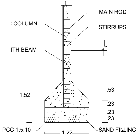
COLUMN DETAILS
