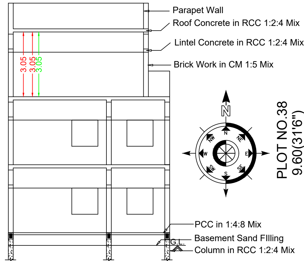
Section RR
