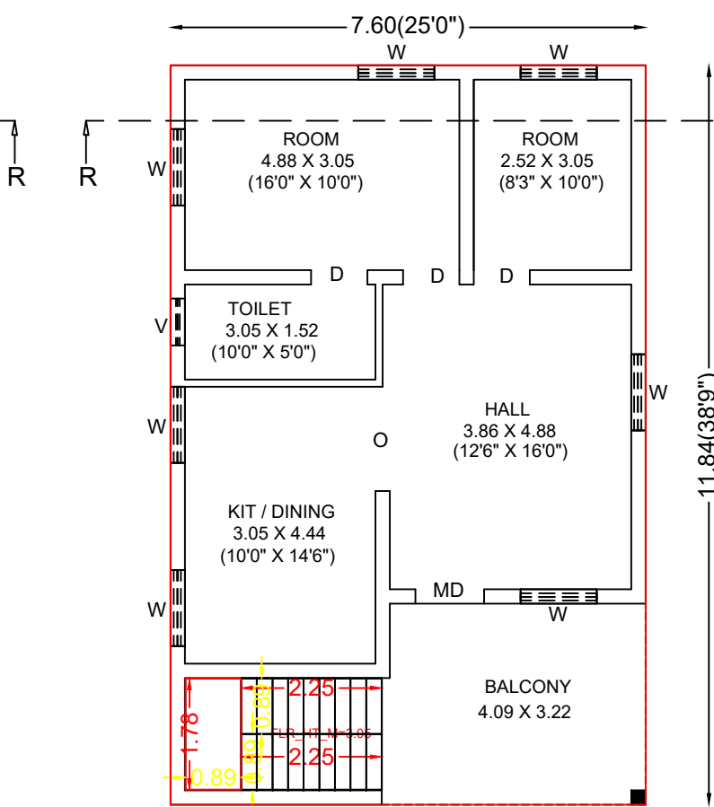
Ex.First Floor Plan
