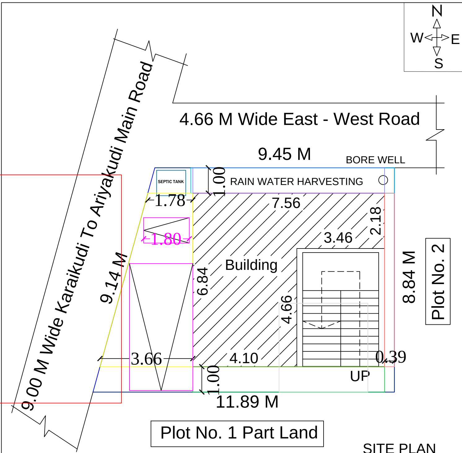
SITE PLAN
