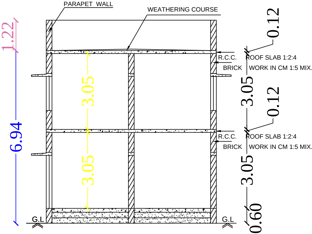
Section on-"AA"
