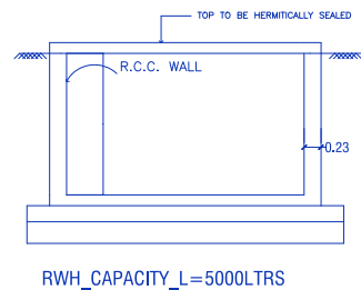
RWH_CAPACITY_L=5000LTRS
