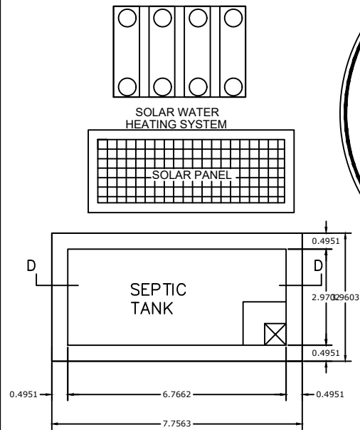
PLAN OF SEPTIC TANK SCALE 1"=2'0"
