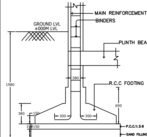
TYPICAL SECTION OF R.C.C COLUMN FOUNDATION SCALE : 1" = 2'-0"
