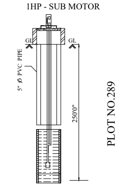
BOREWELL DETAILS
