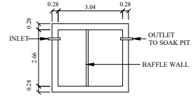
PLAN SEPTIC TANK
