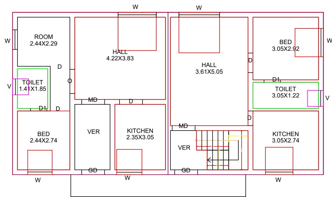
1 FLOOR PLAN
