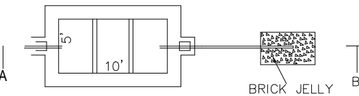
SEPTIC TANK & DISPERSION TRENCH DETAILS SCALE- 1:100
