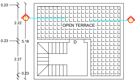
TERRACE FLOOR
