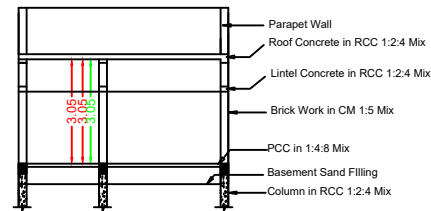
Section RR
