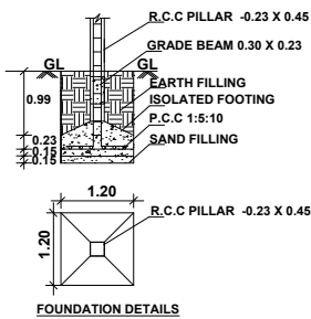
FOUNDATION DETAILS
