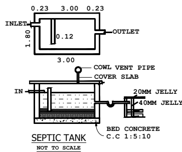
SEPTIC TANK NOT TO SCALE
