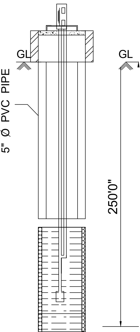
BOREWELL DETAILS
