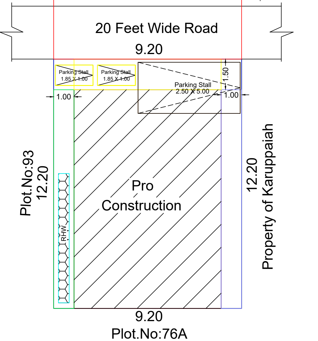
Site Plan
