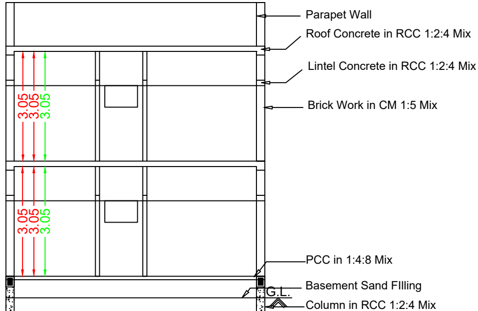
Section RR
