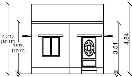
ELEVATION ON WEST
