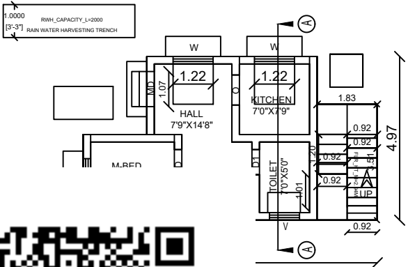
R PLAN
