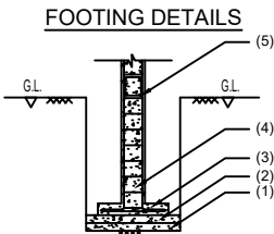
SECTION
