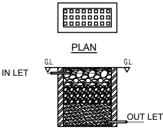
RAINWATER STORAGE PIT DETAILS
